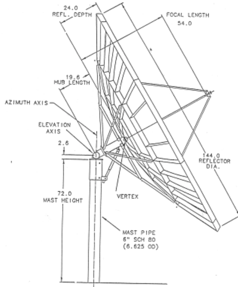
3.7 Meter Series 1374 C-Band Receive Only Axisymmetric Az/EI Antenna Geometry
